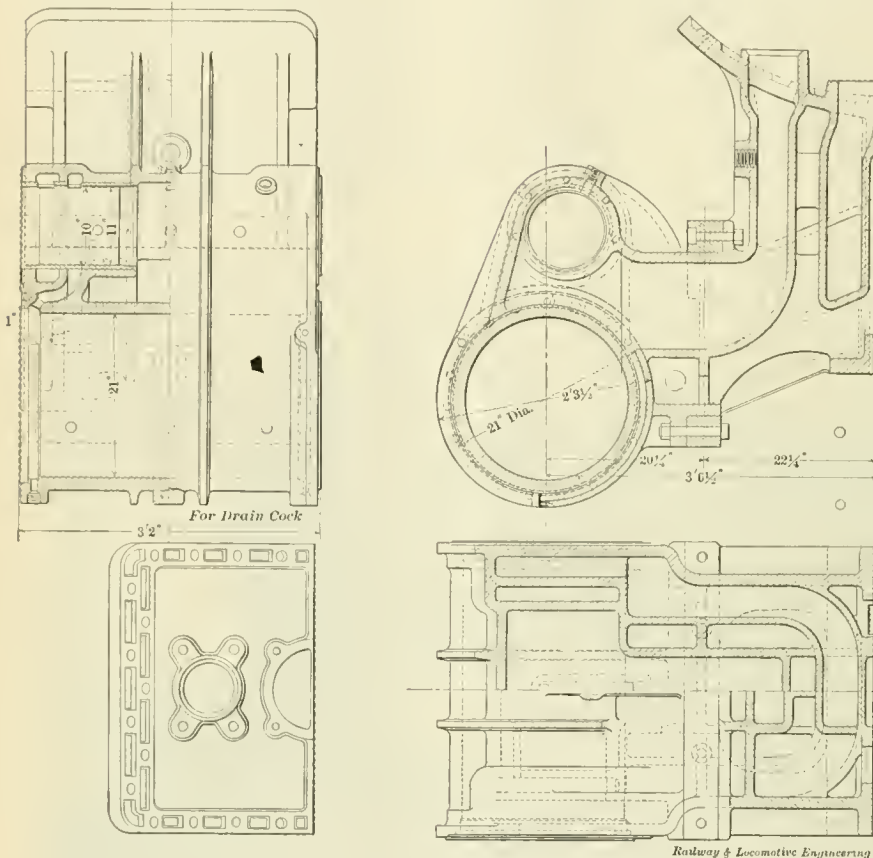
CYLINDER OF NORFOLK &amp; WESTERN CONSOLIDATION.
